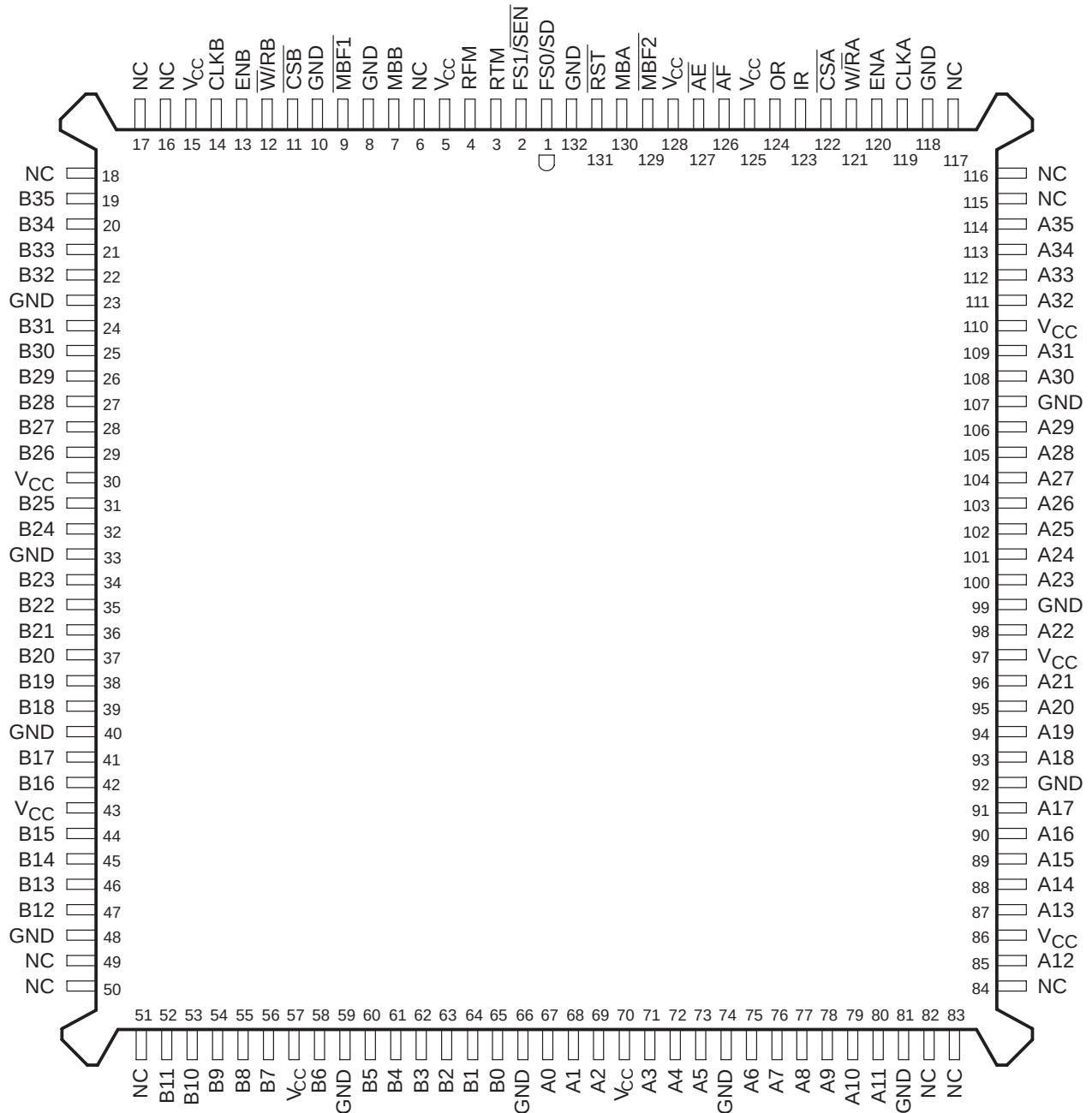
PQ PACKAGE† (TOP VIEW)
